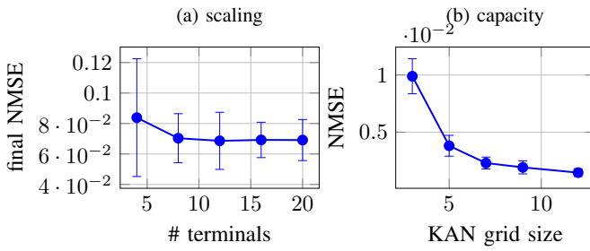
Fig. 8. (a) accuracy improves with more terminals then saturates; (b) under centralized abundant data a larger grid keeps helping. In the data-limited federated regime, however, growing the grid online overfits (Sec. VI), so a fixed modest grid is preferred.
