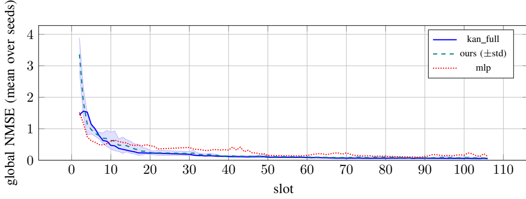
Fig. 4. Convergence and tracking under drift: NMSE vs. slot averaged over all seeds (shaded band = \pm std for the proposed method). The KAN advantage is consistent across seeds and across the entire non-stationary horizon, and the proposed sparsified variant tracks the dense KAN at half the uplink.
