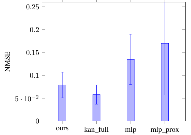
Fig. 3. NMSE (mean±std, ten seeds). Both KAN variants are well below the MLPs.
