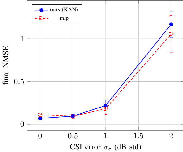
Fig. 10. CSI estimation error in the federated loop (a boundary study). The KAN leads only at \sigma_c \approx 0 ; from \sigma_c \geq 0.5 the MLP is comparable or marginally better, and both degrade together at large error.
