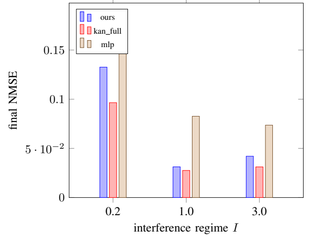
Fig. 9. Final NMSE per interference regime. The KAN advantage holds across the drift range, not just on average.
