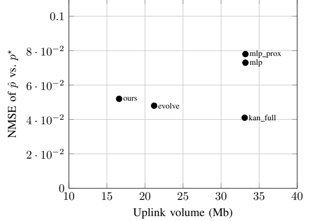
Fig. 2. Communication–accuracy frontier. The proposed bandit-sparsified KAN (ours) dominates both MLP variants and halves the uplink of the dense KAN.
