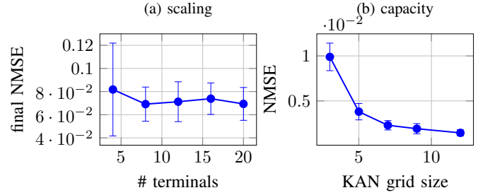
Fig. 8. (a) accuracy improves with more terminals then saturates; (b) under centralized abundant data a larger grid keeps helping. In the data-limited federated regime, however, growing the grid online overfits (Sec. VI), so a fixed modest grid is preferred.
