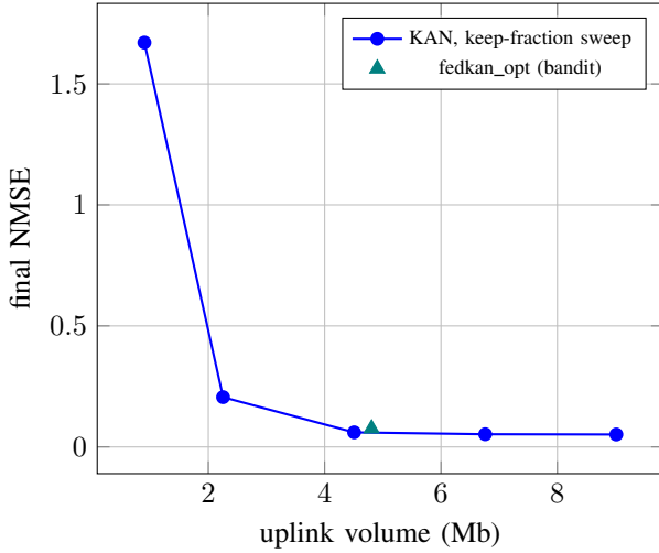
Fig. 7. Communication-accuracy frontier from a keep-fraction sweep; the bandit controller lands on a favorable knee automatically.
