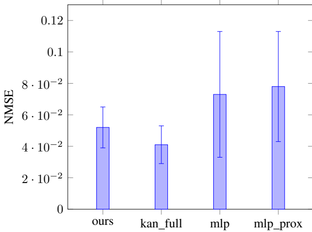
Fig. 3. NMSE (mean \pm std, 20 seeds). Both KAN variants are well below the MLPs.
