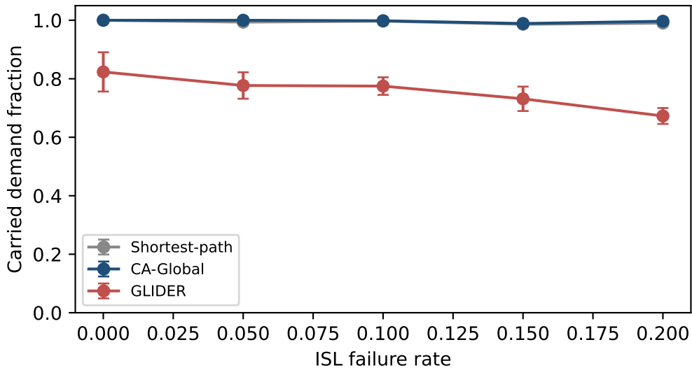
Robustness to link churn (Starlink-like)
