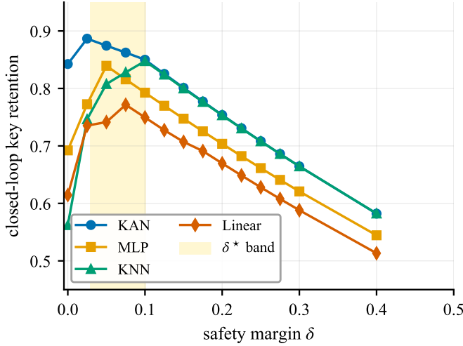
Fig. 5. \beta safety-margin deployment recipe: closed-loop key retention vs the scalar safety margin \delta applied as \beta_{\text{deploy}} = \hat{\beta} + \delta . The unimodal shape and the model-agnostic peak in [0.03, 0.10] make \delta^* a single-knob deployment dial. KAN: 0.84 \rightarrow 0.89; KNN: 0.56 \rightarrow 0.83.
