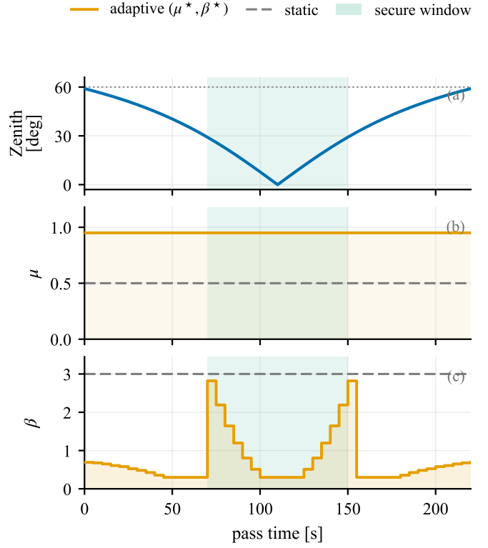
Fig. 6. Single-link adaptive control over a LEO pass. Top: zenith trajectory. Middle/bottom: adaptive \mu^*, \beta^* (orange step) vs static (grey dashed). The \beta^* envelope is well-fit by the closed-form rule (21), justifying the KAN interpretability claim; the \mu^* envelope saturates near \mu_{\max} except where Eve binds.
