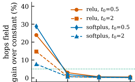
released: width 16, 3 layers
