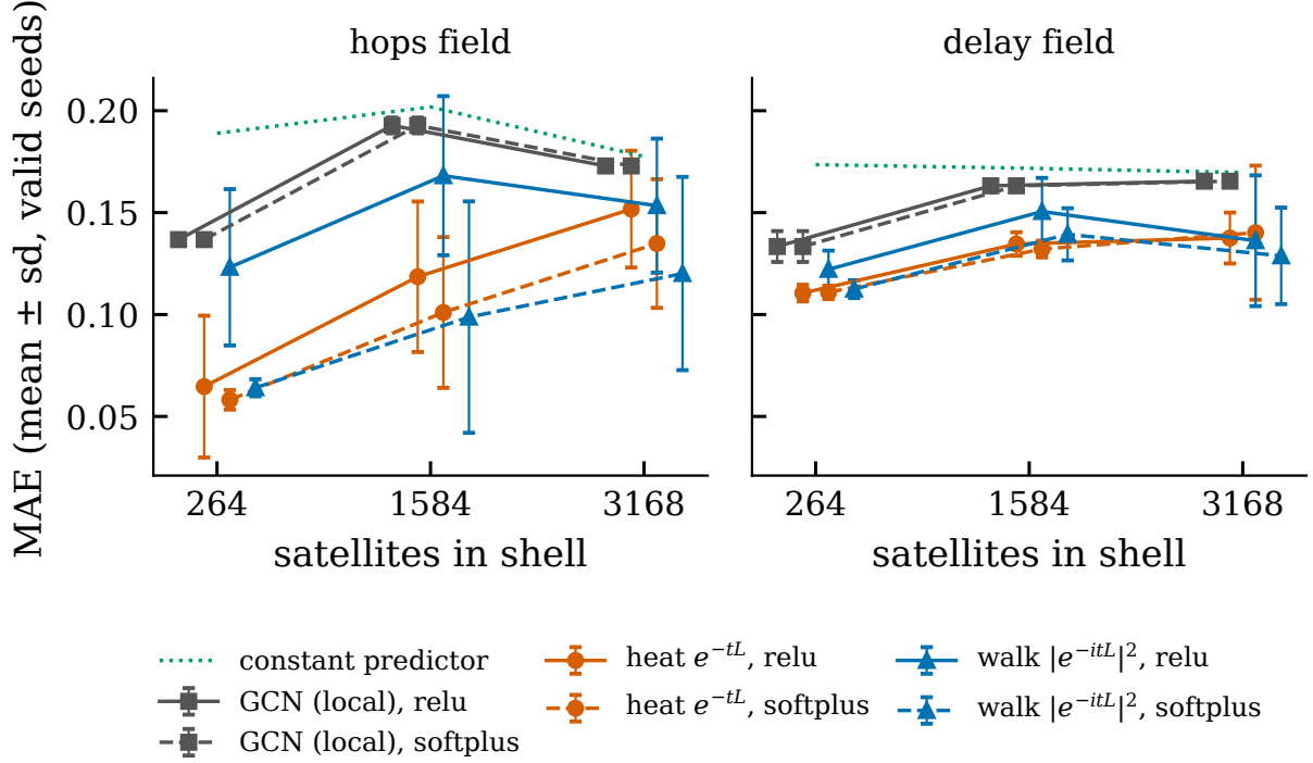
Figure 6: MAE against shell size at 1000 epochs, submitted capacity, both t arms, both tasks. Points are means over valid seeds and bars one standard deviation; the dotted line is the constant predictor. Points are offset horizontally within each shell for legibility.
