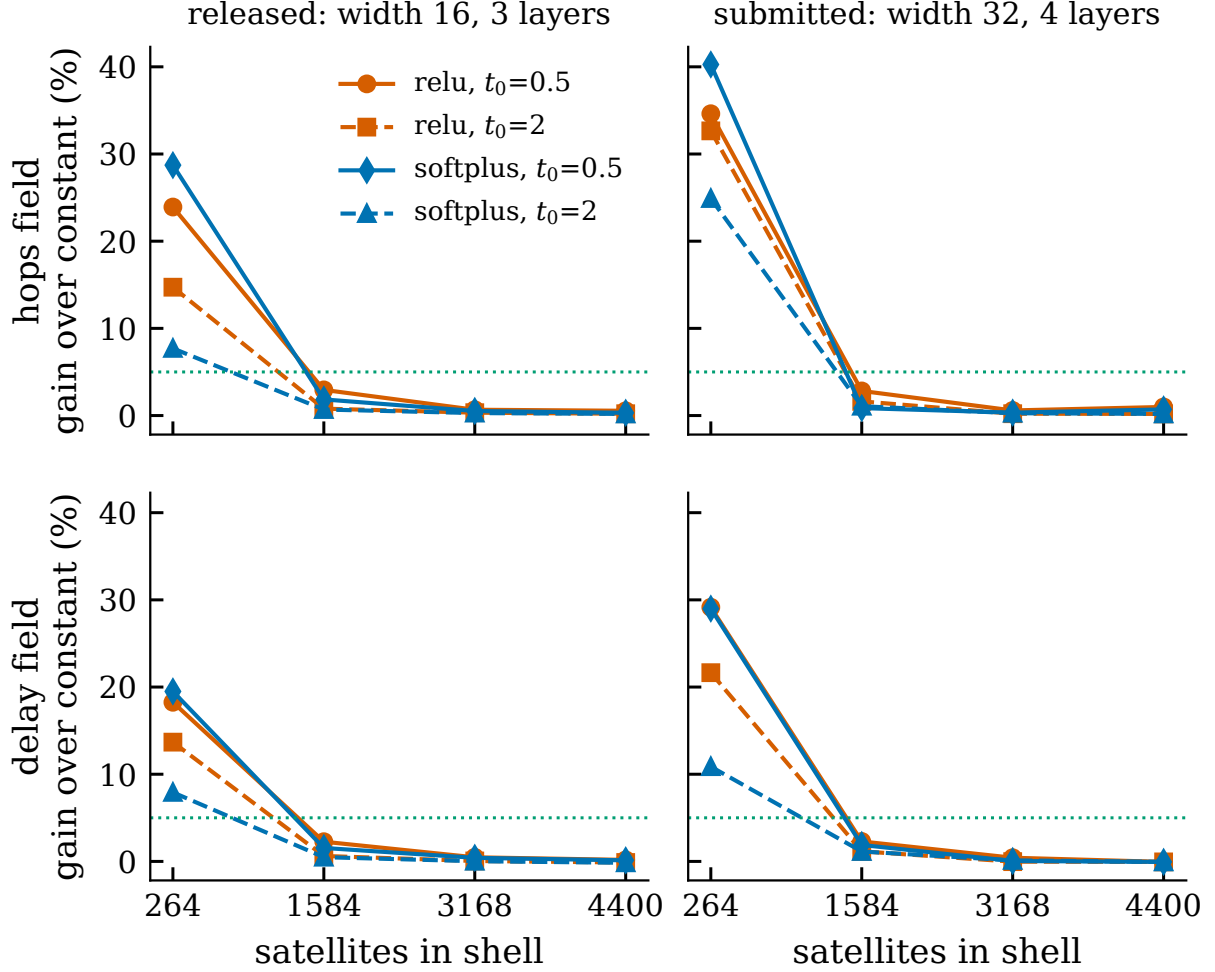
Figure 3: Gain (5) of the best operator over the constant predictor at 200 epochs, as a function of shell size, for the hop field (top) and the delay field (bottom), the released and the submitted capacity (columns) and the four t arms. The dotted line is the 5% floor of rule 3. Above 264 satellites every combination lies below it on both tasks.
