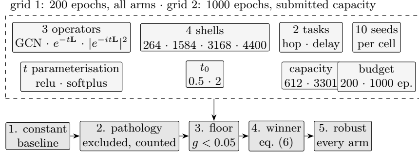
Figure 2: The study design. Every cell of the grid, one (task, shell, arm), runs the three operators on the same instances and seeds; the five reading rules are applied in order by one script, and a ranking is reported only if it survives all five.
