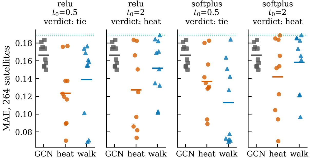
Figure 4: Per-seed MAE on the hop field, 264 satellites, submitted capacity, 200 epochs, for the four t arms. Bars are means over valid seeds; the dotted line is the constant predictor. The two spectral operators are bimodal across seeds: a run either leaves the constant solution or stays near it.
