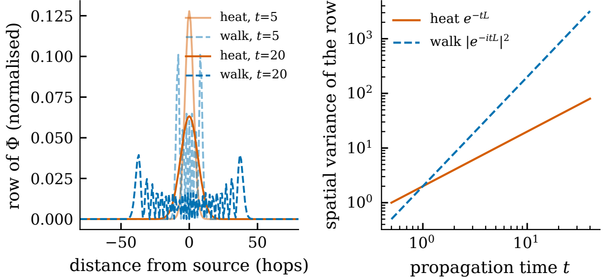
Figure 1: Analytic illustration on a path of 401 nodes. Left: one row of the heat kernel and of the walk kernel from the central node at two propagation times, normalised to sum to one. Right: spatial variance of the row against t on logarithmic axes; the fitted slopes are 1.00 for the heat kernel and 2.00 for the walk kernel.
