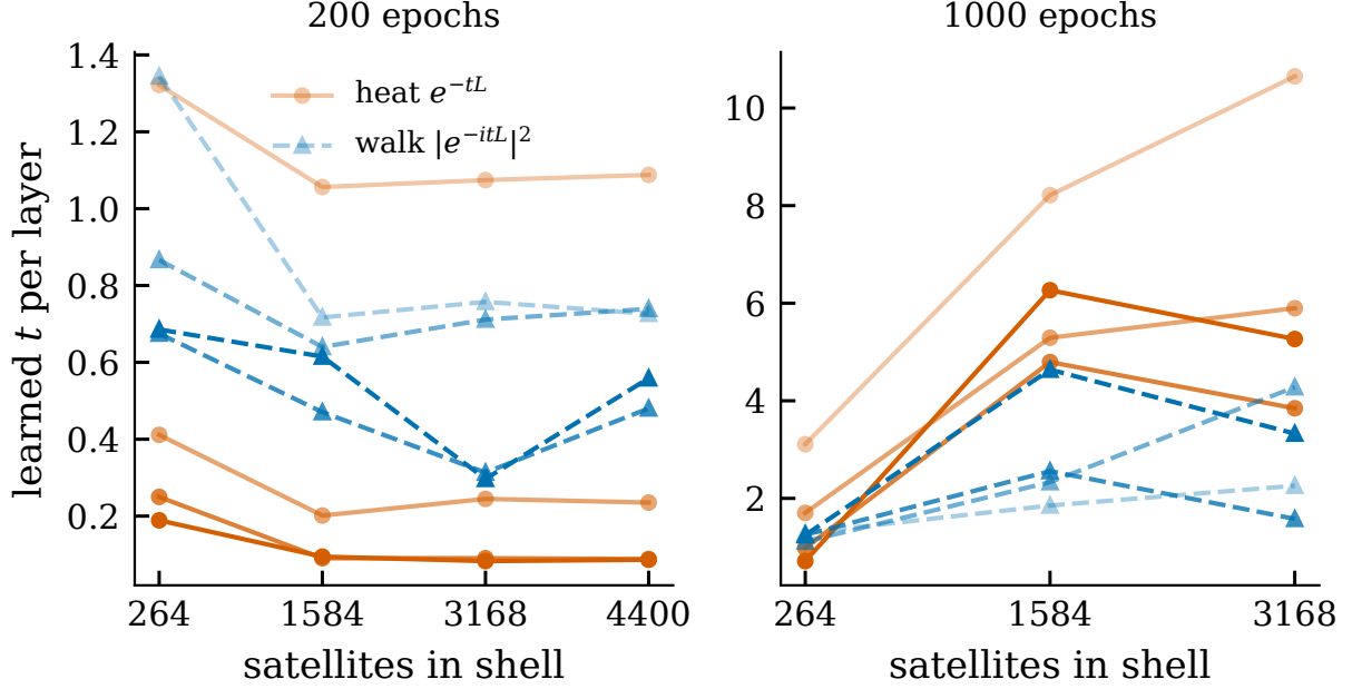
Figure 5: Learned propagation time per layer (lighter to darker: first to fourth layer) against shell size, hop field, submitted capacity, softplus arm with t_0 = 0.5 , mean over valid seeds. Left: 200 epochs (grid 1). Right: 1000 epochs (grid 2). Note the different vertical scales.
