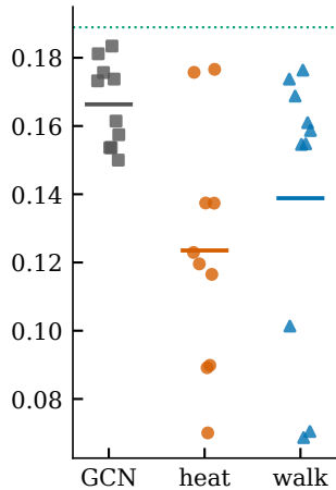
MAE, 264 satellites
