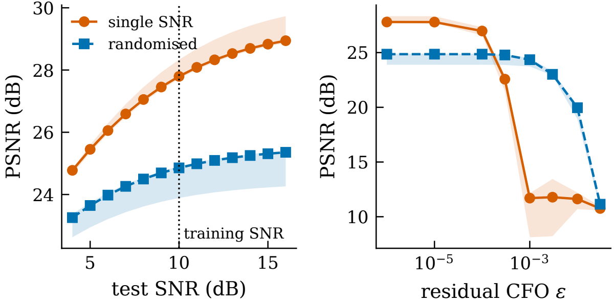
Figure 7: A codec trained at a single operating point, evaluated across the conditions Section 5 measured. (a) test signal-to-noise ratio; (b) residual normalised frequency offset \varepsilon = f_{\text{res}}/R_s of (11), on a logarithmic axis with the zero-offset case placed at the left edge. “Single SNR” is the fixed-operating-point regime and “randomised” the regime that draws both the signal-to-noise ratio and the offset during training. Bands span 3 seeds.
