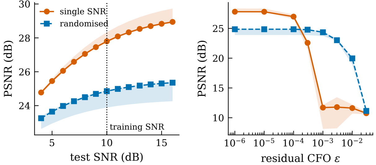
Figure 7: A codec trained at a single operating point, evaluated across the conditions Section 5 measured. (a) test signal-to-noise ratio; (b) residual normalised frequency offset \varepsilon = f_{\text{res}}/R_s of (11), on a logarithmic axis with the zero-offset case placed at the left edge. “Single SNR” is the fixed-operating-point regime and “randomised” the regime that draws both the signal-to-noise ratio and the offset during training. Bands span 3 seeds.
