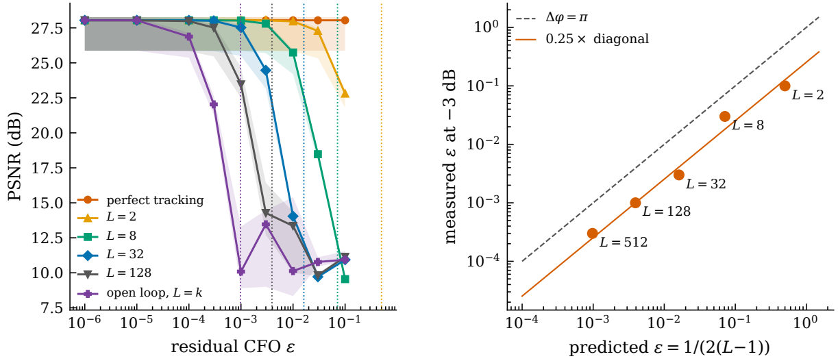
Figure 8: The collapse is governed by accumulated phase, not by Doppler as such. (a) quality against residual offset for four carrier re-estimation intervals, medians over the 7 valid runs of the fixed regime with bands spanning them, dotted verticals marking the position (12) predicts for each L . (b) measured cliff, taken as the first three-decibel loss, against the predicted position; the points lie parallel to the diagonal at 0.25\times .
