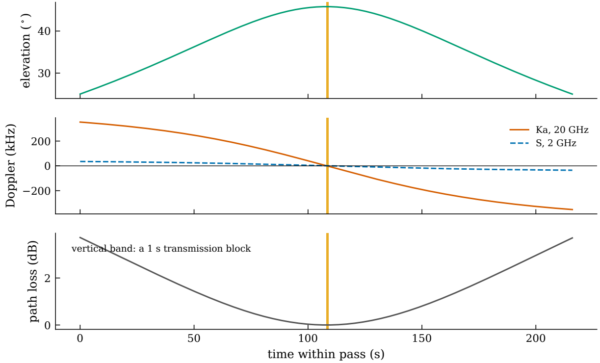
Figure 3: One pass of Starlink 5768 over the station, reaching 45.8^\circ . The selection rule is stated in the text and in the released code. Path loss is plotted relative to its minimum.
