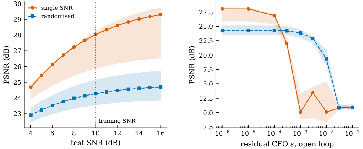
Figure 7: A codec trained at a single operating point, evaluated across the conditions Section 5 measured, over the 7 valid runs of the fixed regime and the 5 of the randomised regime. (a) test signal-to-noise ratio; (b) residual normalised frequency offset of (11) under the open-loop assumption, on a logarithmic axis with the zero-offset case at the left edge. “Single SNR” is the fixed-operating-point regime and “randomised” the regime that draws both quantities during training.
