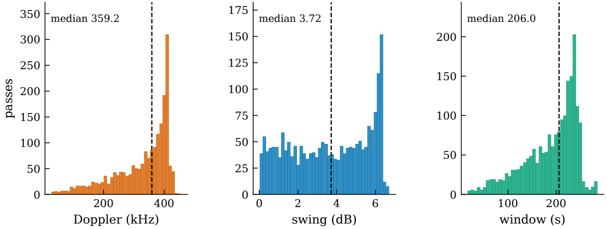
Figure 2: Distributions over 1,978 passes at one station with a minimum elevation of 25^\circ : peak Doppler shift at Ka-band, the swing of the geometric link-budget term across a pass, and the visibility window. Dashed lines mark medians. The spread of the centre panel is explained by geometry rather than assumed to be: swing correlates with maximum elevation at r = 0.962 , and the third of passes that stay lowest sweep a median of 1.20 dB against 6.02 dB for the third that pass highest.
