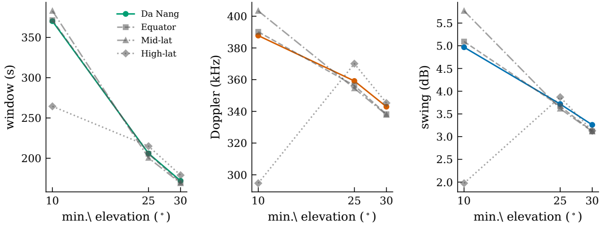
Figure 4: Medians of the same three quantities, visibility window, peak Ka-band Doppler and link-budget swing, against the minimum elevation threshold, for four stations. The station used elsewhere in this paper is drawn in colour and the others in grey; the curves lie close together, which is the same shell property Table 2 reports.
