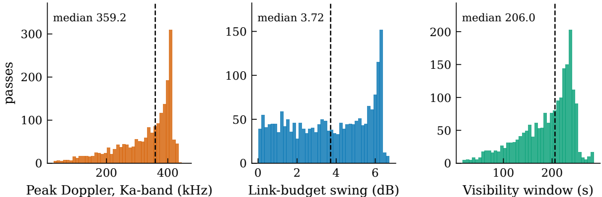
Figure 2: Distributions over 1,978 passes at one station with a minimum elevation of 25^\circ . Dashed lines mark medians. The bimodality of the centre panel reflects the difference between overhead passes, which sweep the full range of slant range, and grazing passes, which do not.
