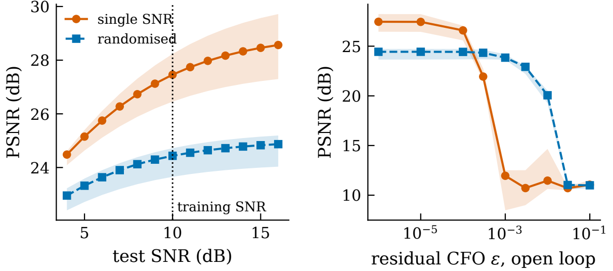
Figure 7: A codec trained at a single operating point, evaluated across the conditions Section 5 measured, over the 4 valid runs of the fixed regime and the 5 of the randomised regime. (a) test signal-to-noise ratio; (b) residual normalised frequency offset of (11) under the open-loop assumption, on a logarithmic axis with the zero-offset case at the left edge. “Single SNR” is the fixed-operating-point regime and “randomised” the regime that draws both quantities during training.
