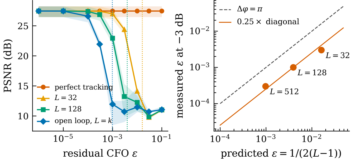
Figure 8: The collapse is governed by accumulated phase, not by Doppler as such. (a) quality against residual offset for four carrier re-estimation intervals, medians over the 4 valid runs of the fixed regime with bands spanning them, dotted verticals marking the position (12) predicts for each L . (b) measured cliff, taken as the first three-decibel loss, against the predicted position; the points lie parallel to the diagonal at 0.25\times .
