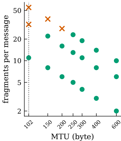
gnutls
