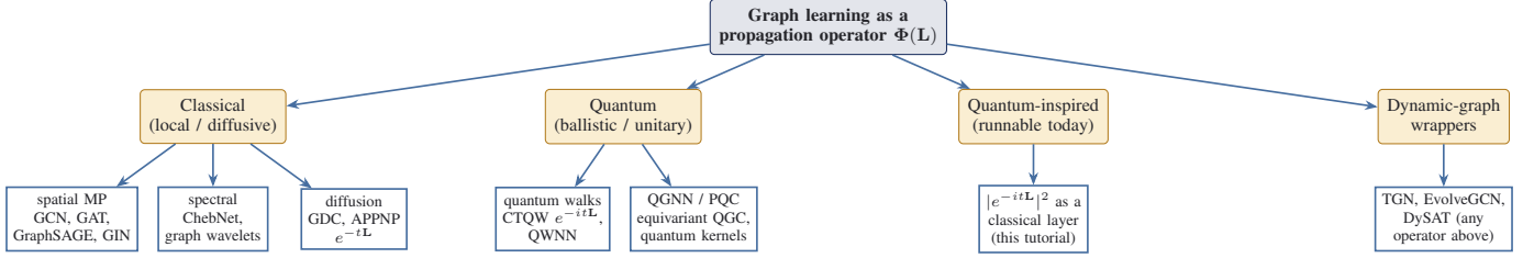
Fig. 3. A taxonomy of graph learning organized by the propagation operator \Phi(\mathbf{L}) . Classical operators are local (spatial message passing) or diffusive (spectral / heat); quantum operators are unitary and ballistic (continuous-time quantum walks, parameterized quantum graph circuits); the quantum-inspired branch runs the quantum-walk kernel on classical hardware; dynamic-graph wrappers compose with any operator to handle a time-varying topology. This tutorial threads the classical, quantum, and quantum-inspired branches onto one axis.
