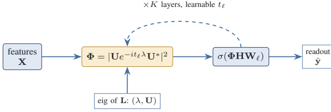
Fig. 5. QI-GNN data flow (Algorithm 1). The quantum-walk kernel is built once from the Laplacian spectrum (fed in from below) and reused across K layers; the heat and GCN variants substitute their operator into the same template, keeping the models param-matched.
