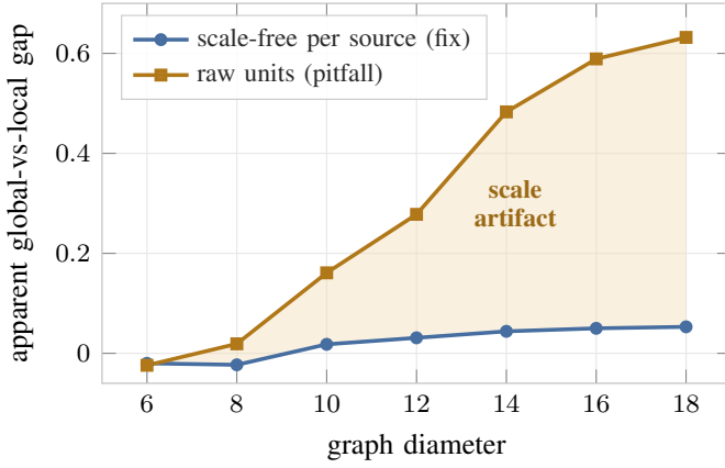
Fig. 12. Exp C1, the normalization pitfall. Pooling errors in raw hop units across graphs of growing diameter manufactures a gap that explodes to 0.63 (slope 0.061). A scale-free per-source normalization leaves a small, genuine gap (slope 0.007, about 9\times flatter): the real long-range deficiency of a local operator, without the scale artifact (shaded).
