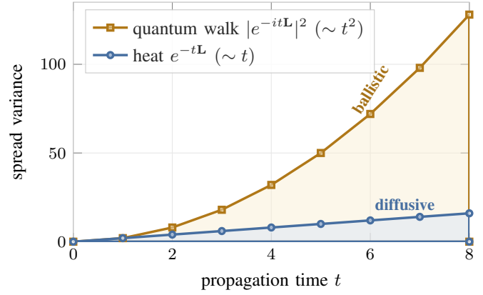
Fig. 7. Exp A, mechanism. Spatial second moment of a propagated impulse on a path graph versus propagation time. Heat diffusion grows linearly ( \text{Var} \sim t ) and the quantum walk ballistically ( \text{Var} \sim t^2 ); a log-log fit gives slopes 1.00 and 2.00, matching (4) and (7). The shaded gap is the quadratic-versus-linear reach advantage.
