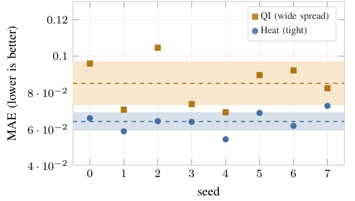
Fig. 13. Exp C2, the single-seed pitfall (66 satellites, 8 seeds). Dashed lines mark the per-operator means and shaded bands the \pm one standard-deviation ranges. The quantum-inspired walk (QI) scatters widely while the heat kernel is tight; a single seed could show QI beating, matching, or losing to heat. Only the distribution, 0.085 \pm 0.012 versus 0.064 \pm 0.005 , is trustworthy.
