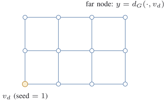
Fig. 6. The node-potential task. A single seeded signal at the destination v_d must be propagated across the dynamic LEO graph to recover the geodesic-distance field. The task rewards long-range operators and exposes a local GCN's K -hop horizon.
