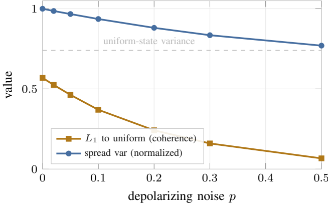
Fig. 10. Exp D, NISQ noise erodes the ballistic mechanism. A continuous-time quantum walk on an 8-node path is run as a PennyLane mixed-state circuit; per-qubit depolarizing noise of strength p drives the coherent walk toward the uniform mixed state. The L_1 distance to uniform falls from 0.57 at p=0 to 0.07 at p=0.5 , and the spread variance decays from its clean value (7.08) toward the featureless uniform-state level (5.25, dashed). This is the near-term caveat behind preferring the classical quantum-inspired surrogate.
