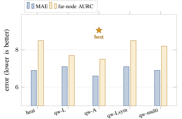
Fig. 9. Exp B2, quantum-walk variant probe (264 satellites, 5 seeds). The base matrix of the walk matters: the adjacency walk (qw-A, starred) is the best operator on both metrics at matched parameters, edging the classical heat kernel on the far-node AURC, while the Laplacian (qw-L) and normalized-Laplacian (qw-Lsym) walks tie heat and the higher-capacity multi-time variant does not improve on qw-A.
