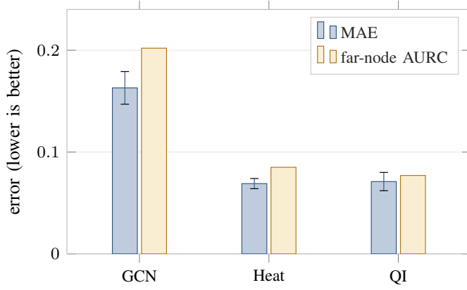
Fig. 8. Exp B, operator comparison on the LEO node-potential task (264 satellites, 5 seeds, param-matched). Global operators (Heat, QI) beat the local GCN by roughly 2.3\times . Heat and the quantum-inspired (QI) walk tie on MAE within the seed spread (error bars); QI shows a small, theory-consistent edge only on the far-node AURC.
