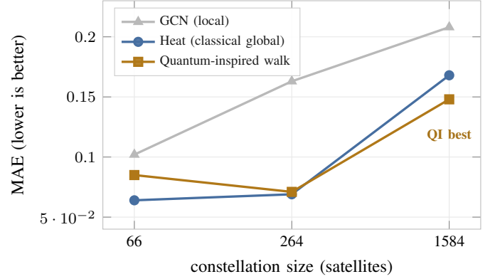
Fig. 11. Exp E, the quantum-inspired edge emerges at scale. Operator MAE versus constellation size at a fixed training budget. The quantum-inspired walk (amber) starts worse than the classical heat kernel (blue) at 66 satellites, ties at 264, and overtakes it at 1584, where geodesics are longest and the ballistic ( \text{Var} \sim t^2 ) reach of the walk pays off; the local GCN trails at every scale.
