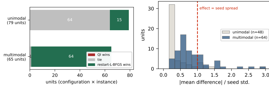
Fig. 2. Left: outcome against restart local search, split by region of the map. Right: distribution of the effect size in units of the seed-induced spread; the dashed line marks the point at which a method difference equals the spread produced by changing the seed alone.
