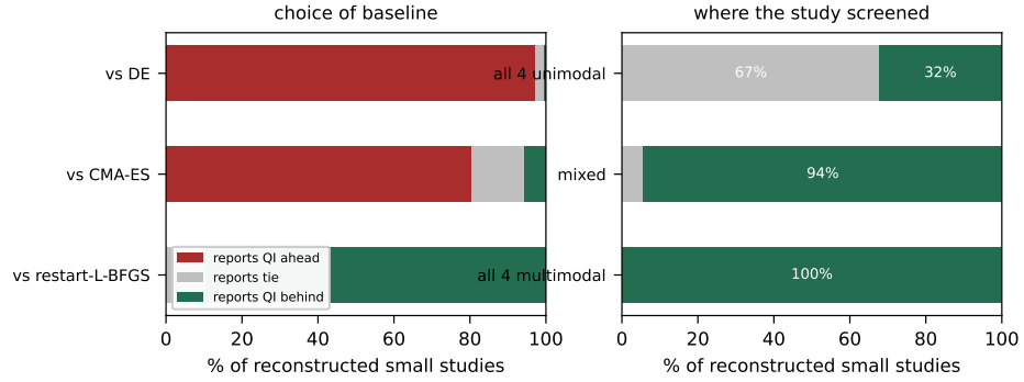
Fig. 3. Verdicts of 5.000 reconstructed studies at the size usually reported. Left: the verdict as a function of which baseline the study chose. Right: the verdict as a function of where in the instance space the study happened to screen.
