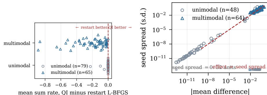
Fig. 4. Left: every one of the 144 units, plotted by the difference in mean sum rate between the QI method and restart local search; no unit falls to the right of zero. Right: the same units placed by effect size against seed spread, with the diagonal marking equality. The 32 units in which both methods were deterministic across all 30 seeds are drawn on the lower band rather than dropped.
