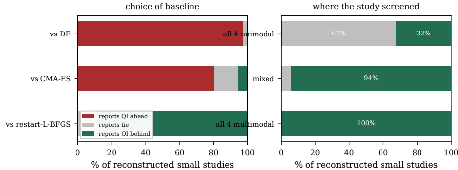
Fig. 5. Verdicts of 5,000 reconstructed studies at the size usually reported. Left: the verdict as a function of which baseline the study chose. Right: the verdict as a function of where in the instance space the study happened to screen.
