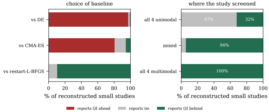
Fig. 5. Verdicts of 5 000 reconstructed studies at the size usually reported. Left: the verdict as a function of which baseline the study chose. Right: the verdict as a function of where in the instance space the study happened to screen.
