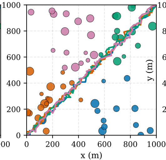
GA
