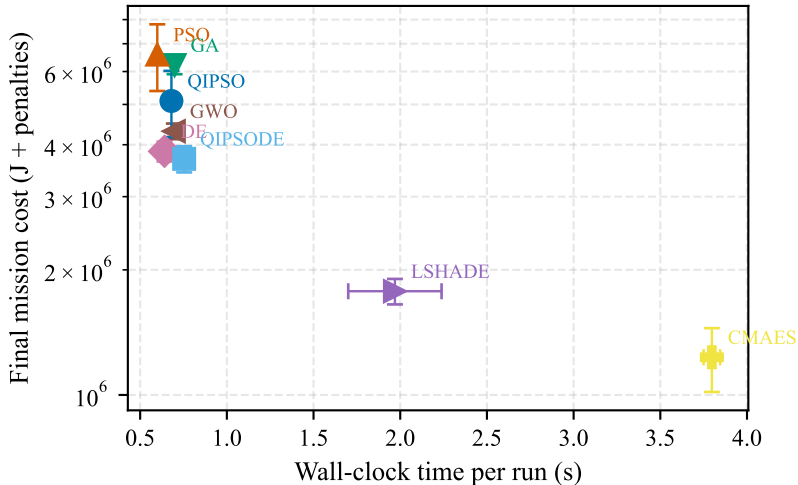
Runtime--cost trade-off, M = 3 , K = 60
