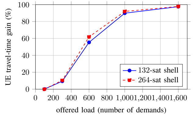
Fig. 4. Congestion headroom: the gain of the user equilibrium over congestion-blind shortest path grows with load, to 98% under heavy load. None at light load.
