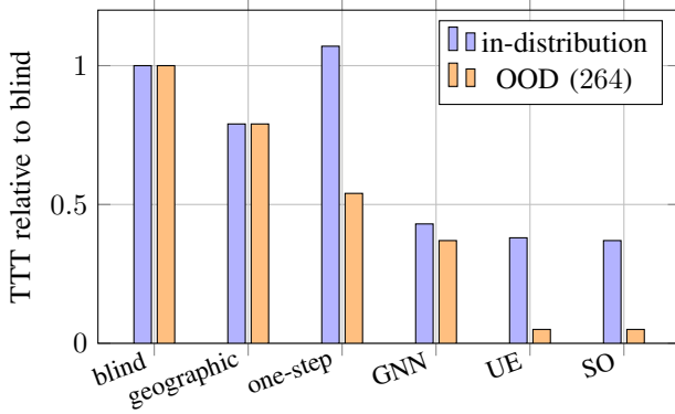
Fig. 5. Travel time relative to blind (lower is better). The GNN approaches UE in distribution and is the best deployable policy out of distribution; the cheap heuristics fail (one-step is worse than blind in distribution, geographic stalls). UE and SO nearly coincide.
