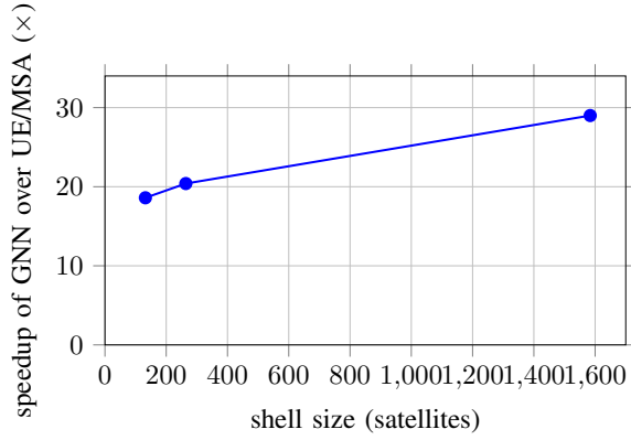
Fig. 6. Inference speedup of the one-shot GNN router over the MSA equilibrium solve, versus shell size. The advantage grows with the constellation.
