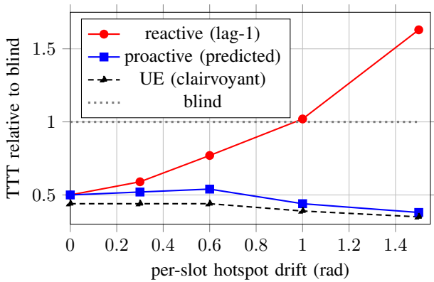
Fig. 7. Proactive versus reactive routing under drifting hotspots. The reactive lag-1 router degrades past blind as the hotspot moves; the proactive router tracks the clairvoyant optimum.
