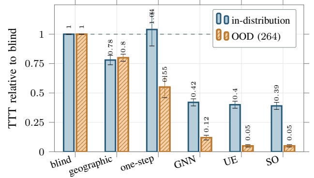
Fig. 5. Travel time relative to blind (lower is better; the dashed line is the blind reference at 1.0). The GNN approaches UE in distribution and is the best deployable policy among the comparators shown here; the cheap heuristics fail (one-step is worse than blind in distribution, geographic stalls). UE and SO nearly coincide.
