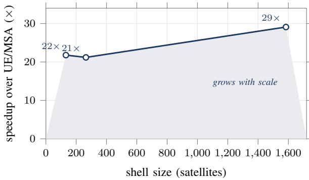
Fig. 3. Inference speedup of the one-shot GNN router over the MSA equilibrium solve, versus shell size. The advantage grows with the constellation, reaching 29 \times at 1584 satellites.
