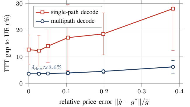
Fig. 2. Travel-time gap to UE against injected price error. The gap grows monotonically and flattens to a floor \delta_{\text{dec}} as the error vanishes, which is the shape Proposition 1 predicts. It is not a validation of the bound: Section IV-F shows the numerical bound is vacuous at every operating point measured here.
