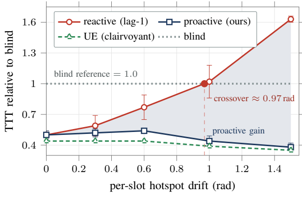
Fig. 8. Proactive versus reactive routing under drifting hotspots (shaded band is the proactive advantage). The reactive lag-1 router degrades past the blind reference once the drift exceeds about one radian; the proactive router tracks the clairvoyant optimum throughout.
