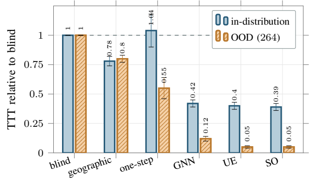
Fig. 5. Travel time relative to blind (lower is better; the dashed line is the blind reference at 1.0). The GNN approaches UE in distribution and is the best deployable policy out of distribution among the comparators shown here; the cheap heuristics fail (one-step is worse than blind in distribution, geographic stalls). UE and SO nearly coincide.
