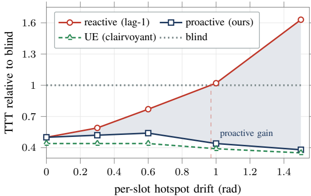
Fig. 7. Proactive versus reactive routing under drifting hotspots (shaded band is the proactive advantage). The reactive lag-1 router degrades past the blind reference once the drift exceeds about one radian; the proactive router tracks the clairvoyant optimum throughout.
