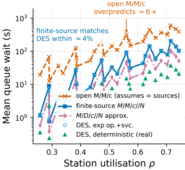
Fig. 3. Queue-model validation against discrete-event simulation. The finite-source model matches the DES under matched (exponential) assumptions and empirically overestimates the wait of the real near-deterministic system on every configuration tested, which is an observation on those configurations and not a proven bound, whereas the open M/M/c overpredicts the wait about 6\times .
