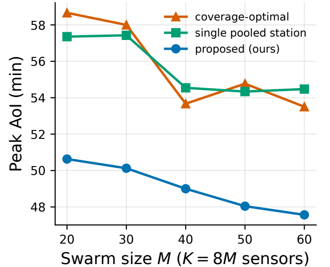
Fig. 7. Scaling to a large swarm ( M up to 60, K = 8M sensors, capacity C_{\text{tot}} = \lceil M/3 \rceil growing with the swarm). The proposed placement keeps its advantage over the baselines at scale. All numbers at this field size assume idealized recharge reachability: constraint (12c) is not met by the returned designs at L > 6 km (Table V), so they should be read as a study of the placement problem rather than of a flyable deployment.
