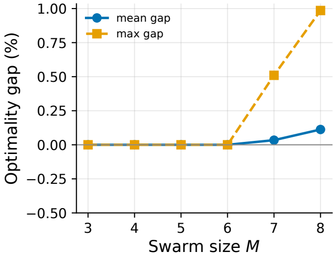
Greedy solver vs exact optimum
