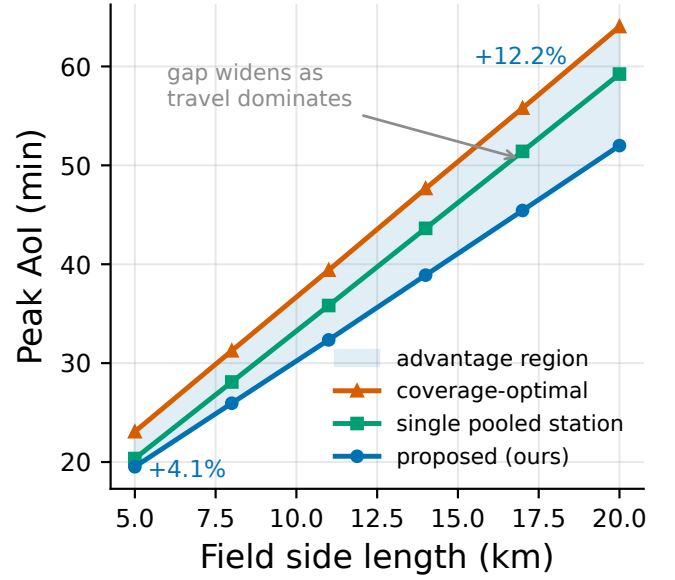
Fig. 6. Field-size sweep. The proposed distributed placement beats the single pooled station at all sizes, with a widening margin as travel cost grows.
