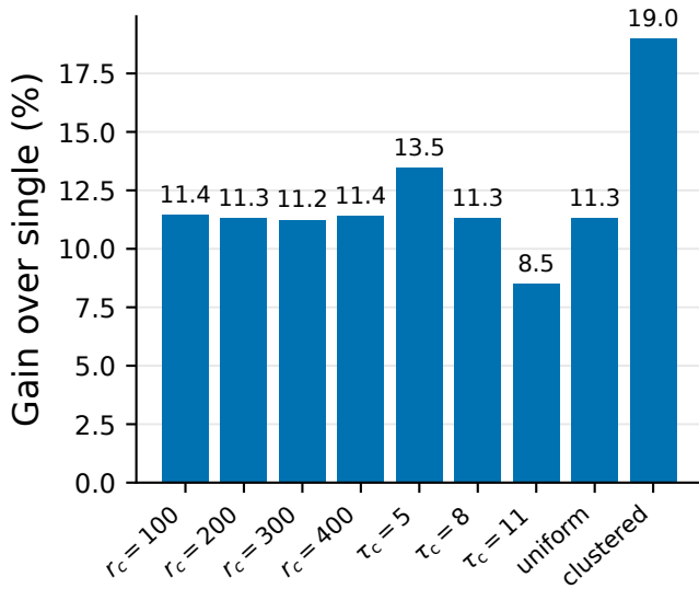
Fig. 8. Robustness of the proposed method's gain over the single pooled station to the collection radius r_c , the charge time \tau_{\text{charge}} , and a uniform versus clustered sensor field ( L = 14 km, M = 12 ).
