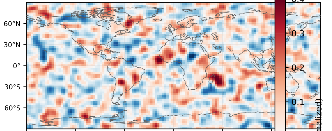
T850 error at +24 h (normalized)
