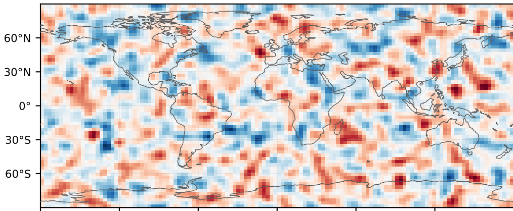
Z500 error at +24 h (normalized)
