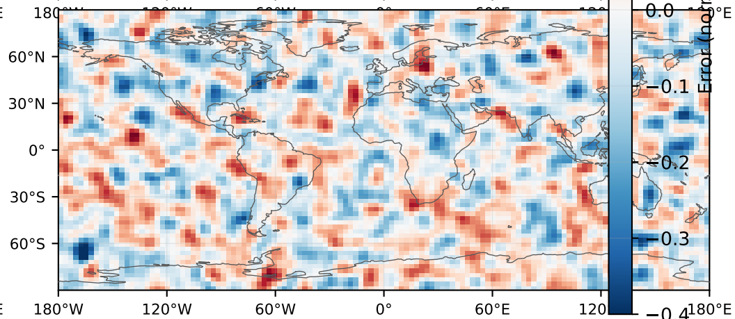
V850 error at +24 h (normalized)
