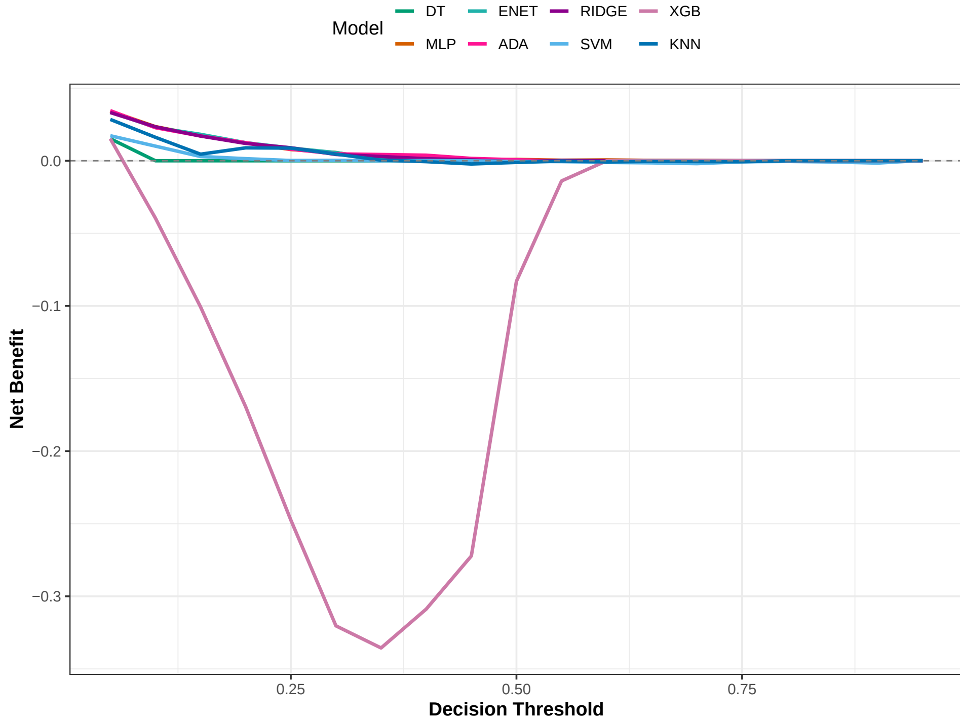
Net Benefit Analysis by Threshold
