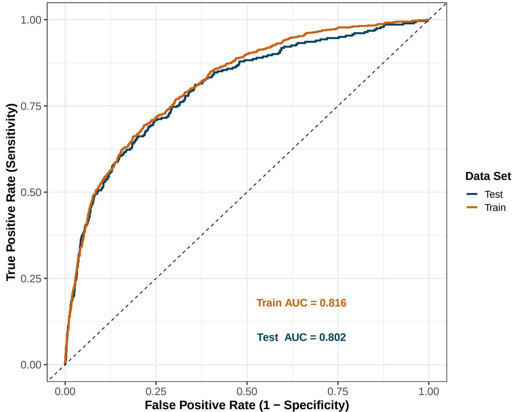
ENET ROC Curve (Train vs Test)
