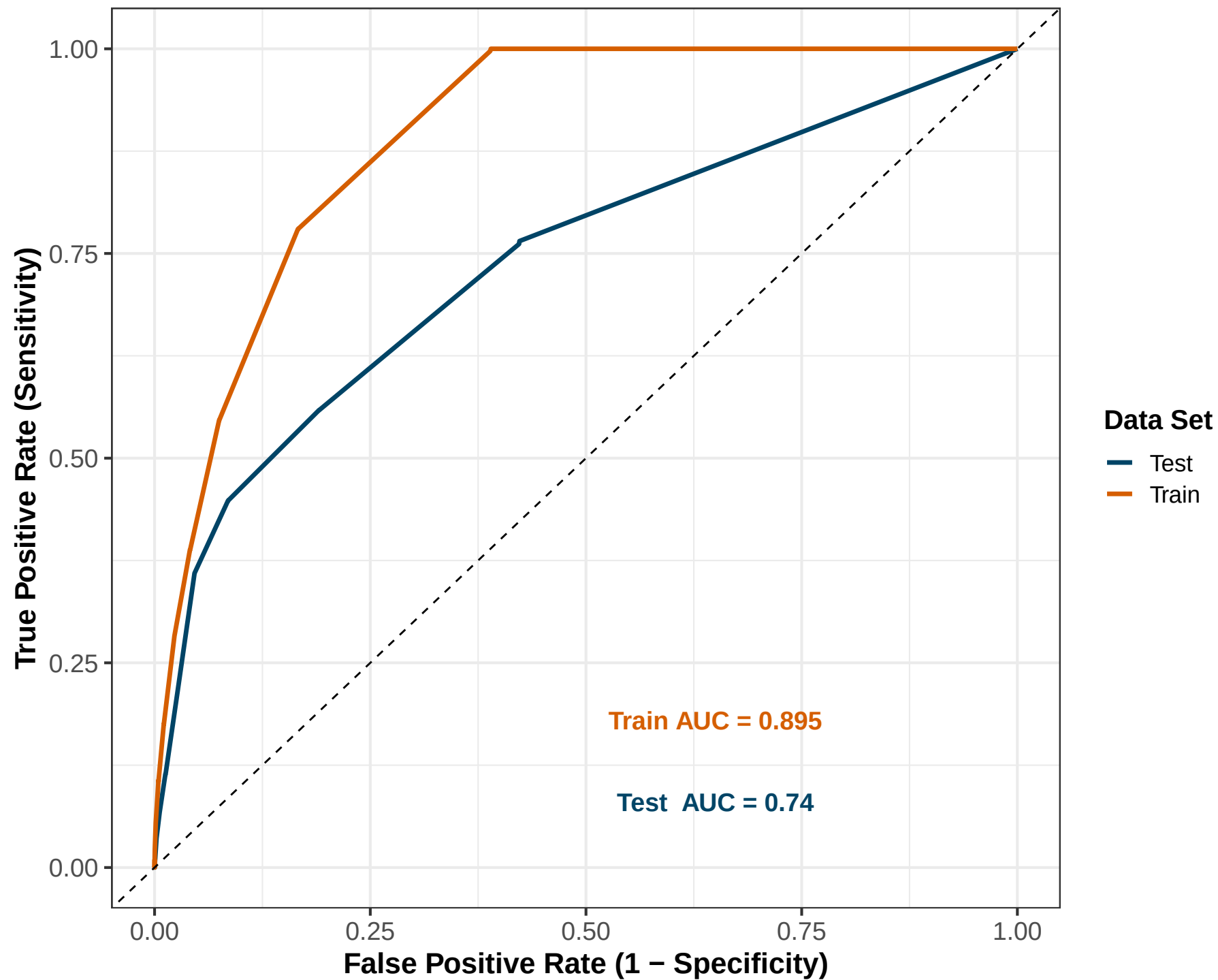
KNN ROC Curve (Train vs Test)
