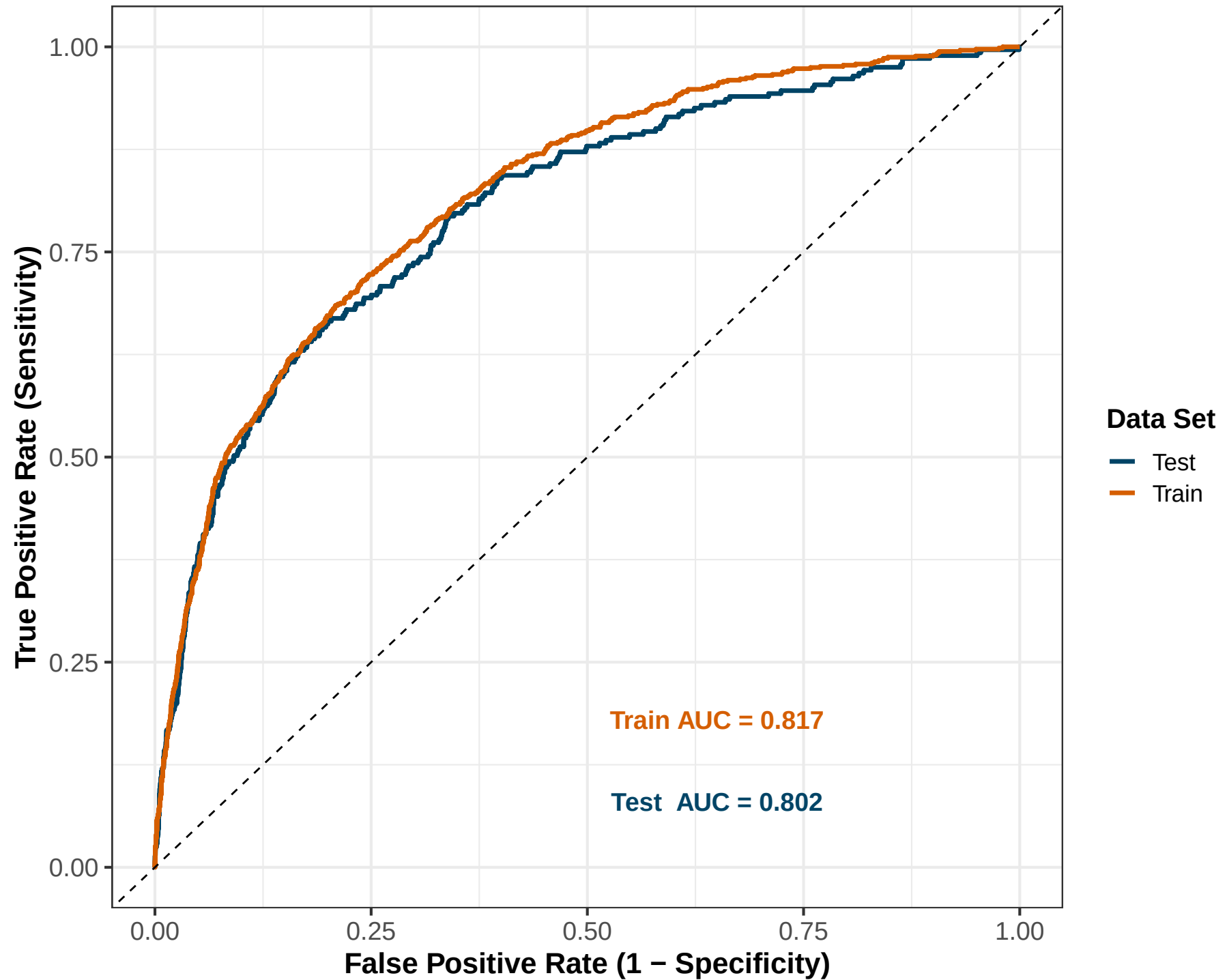
MLP ROC Curve (Train vs Test)
