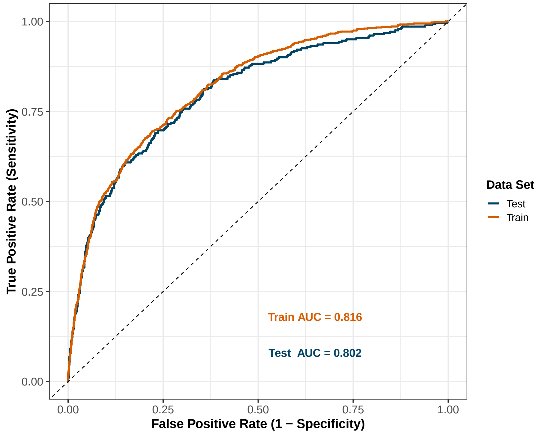
RIDGE ROC Curve (Train vs Test)
