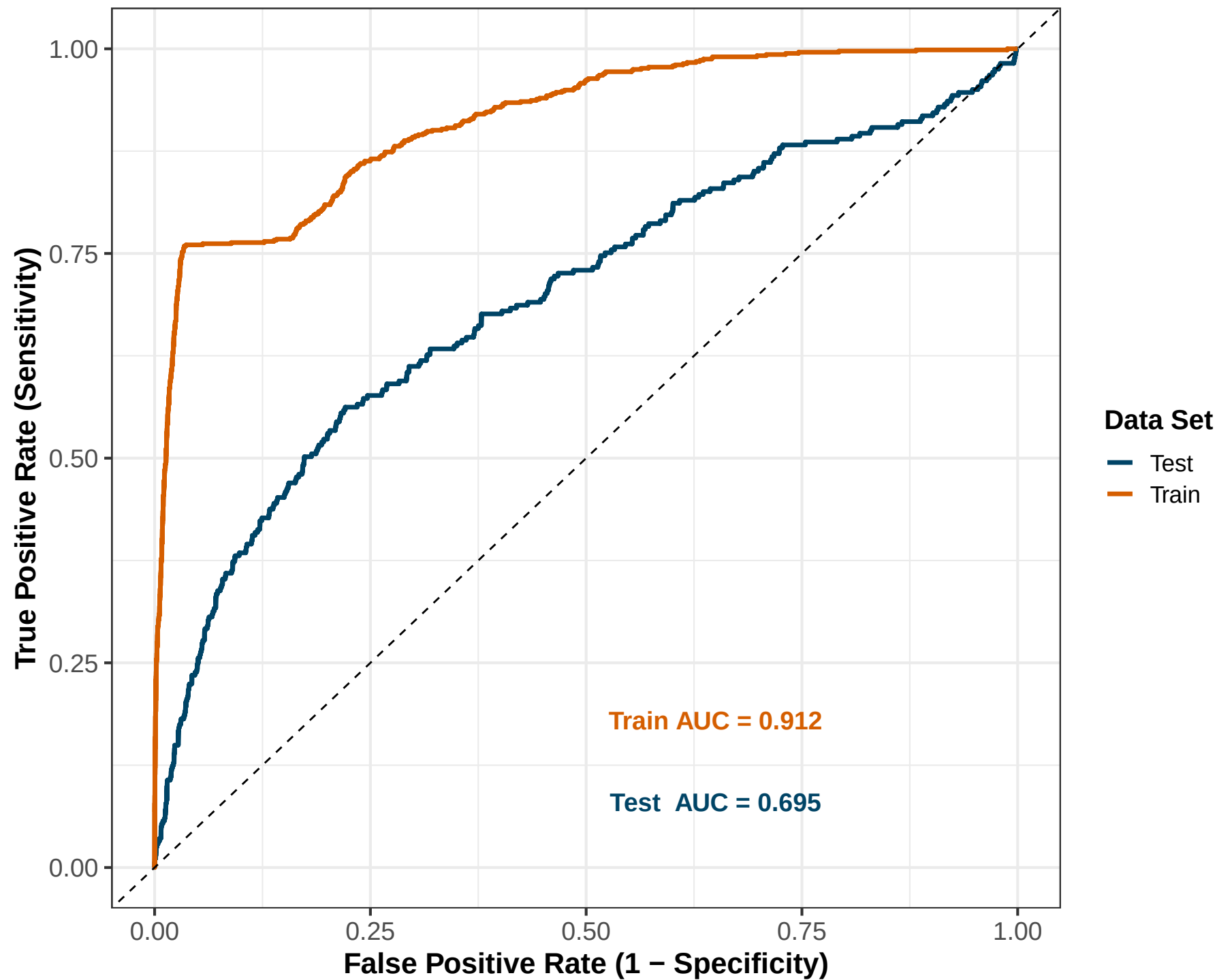
SVM ROC Curve (Train vs Test)
