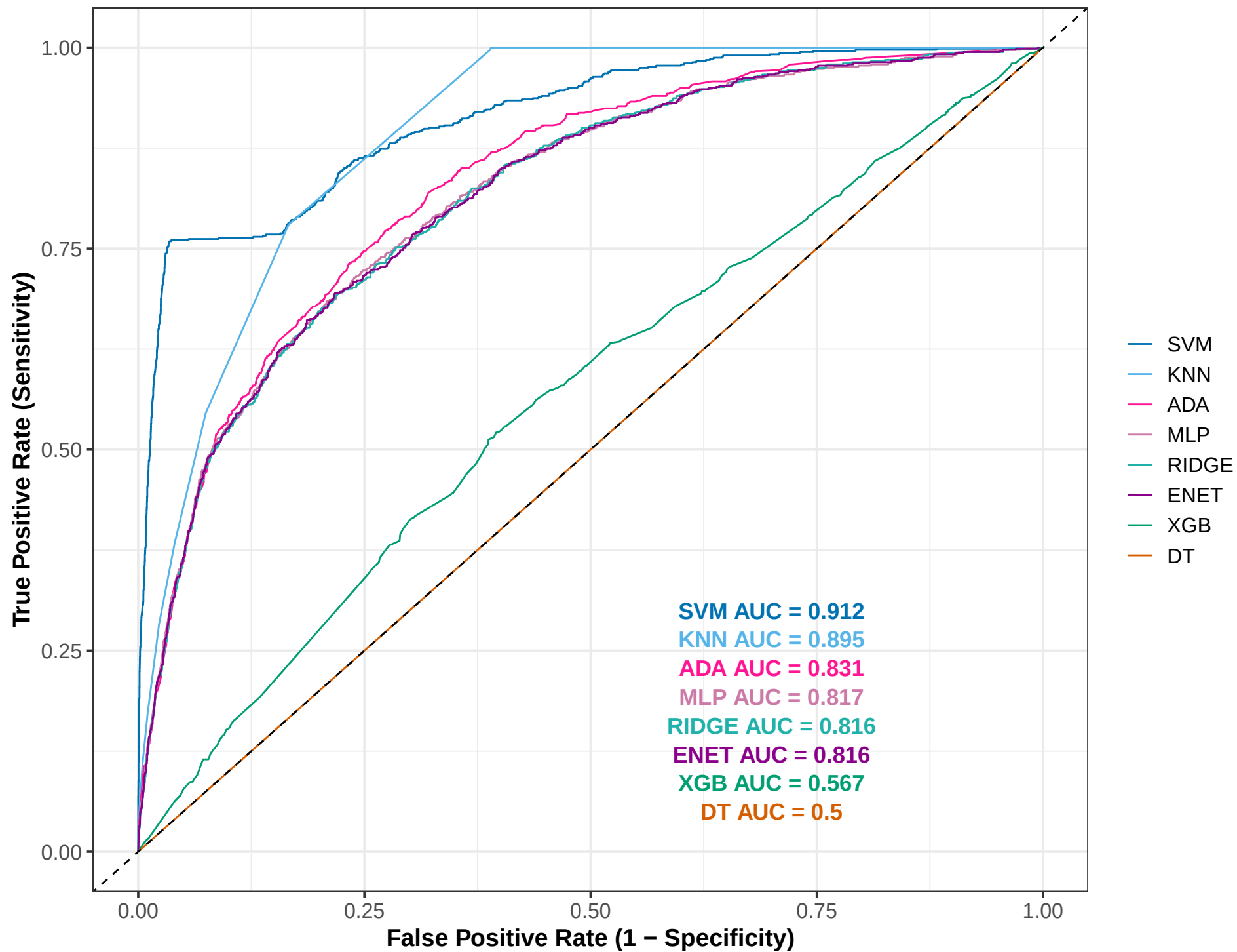
Training Set ROC Curves
