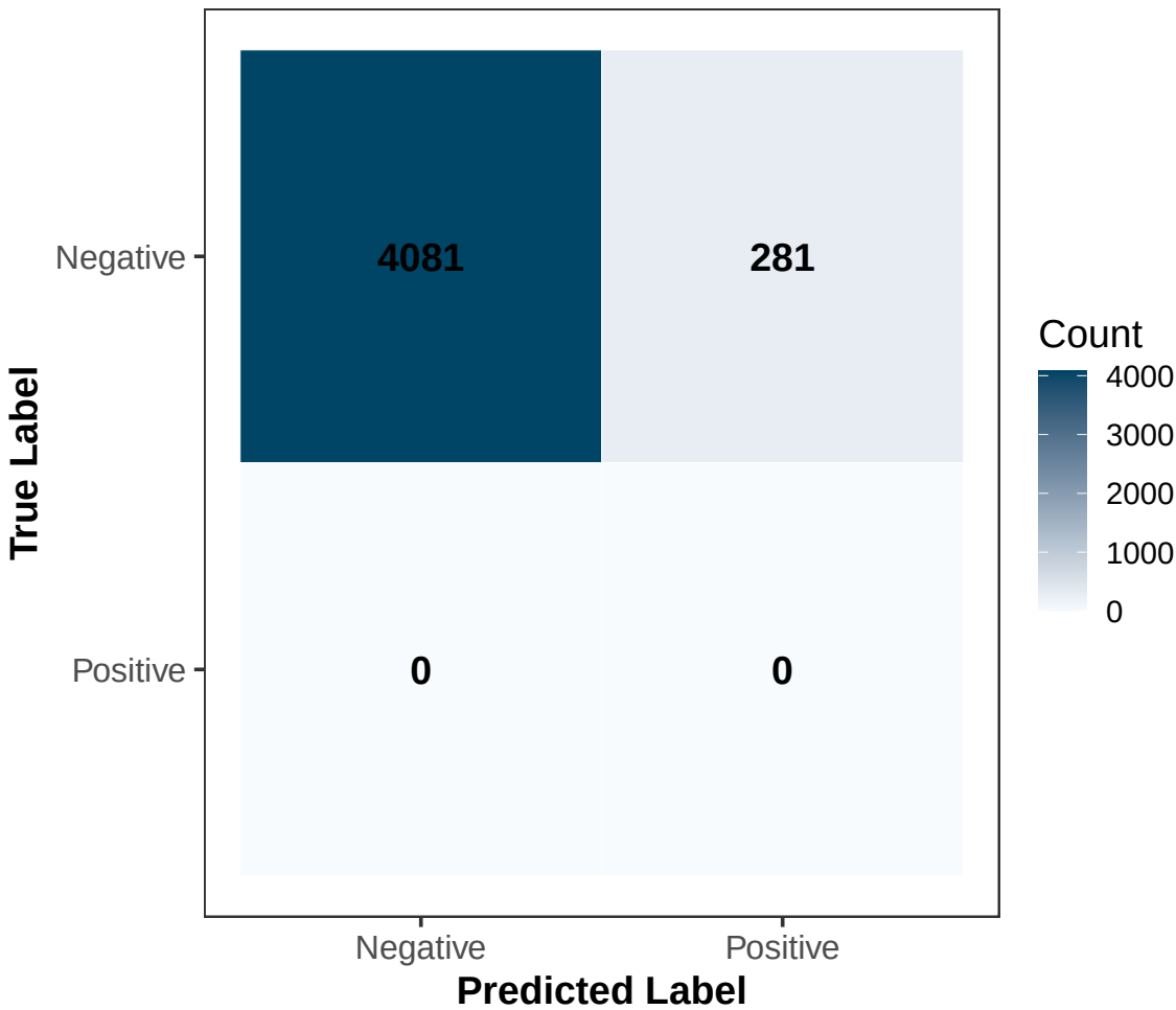
DT Confusion Matrix
