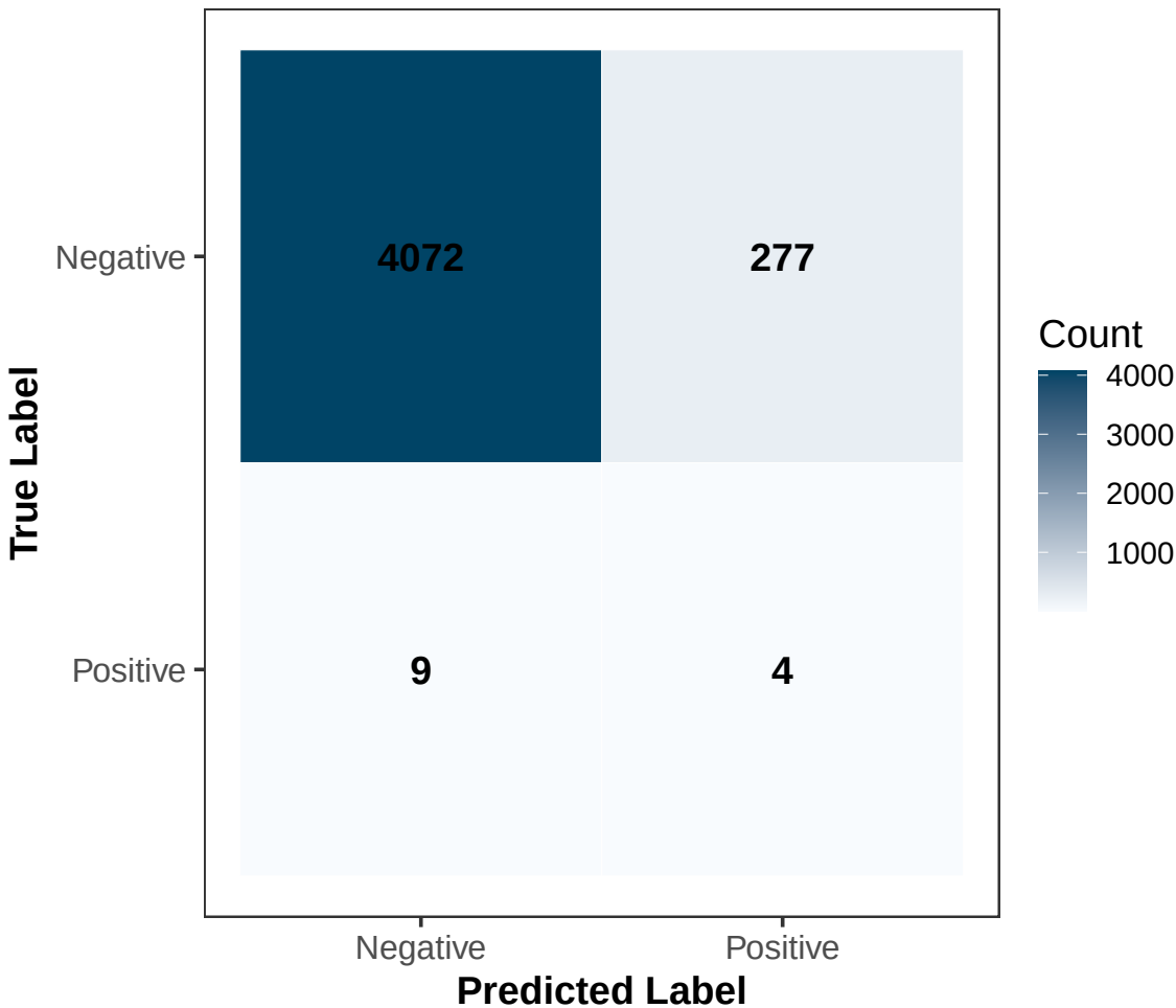
ENET Confusion Matrix
