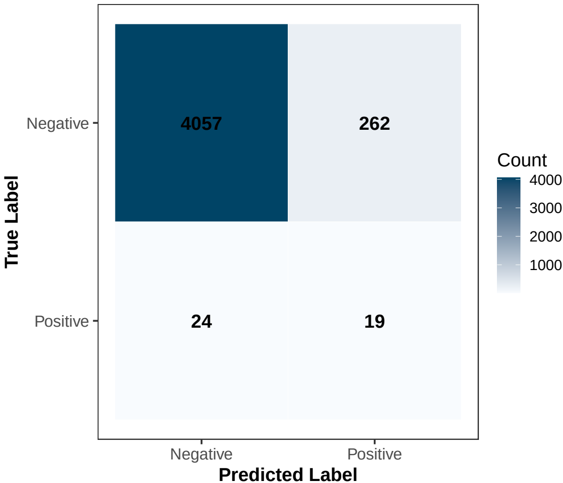
KNN Confusion Matrix
