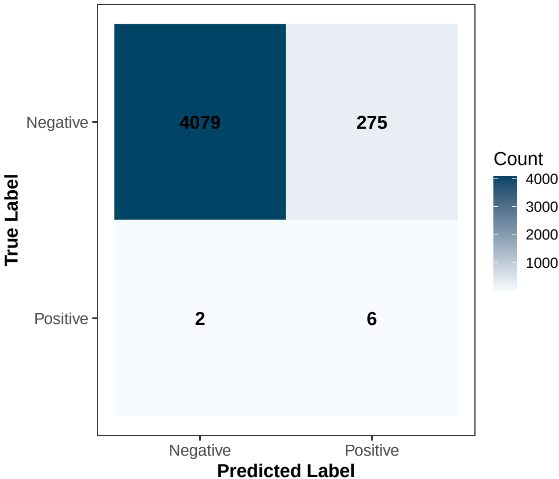
MLP Confusion Matrix
