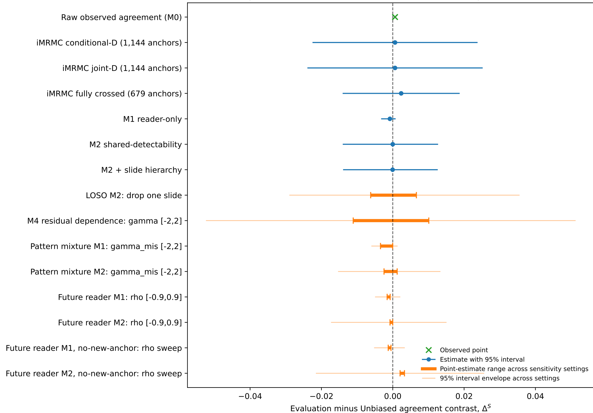
Agreement contrast across models and structural perturbations
