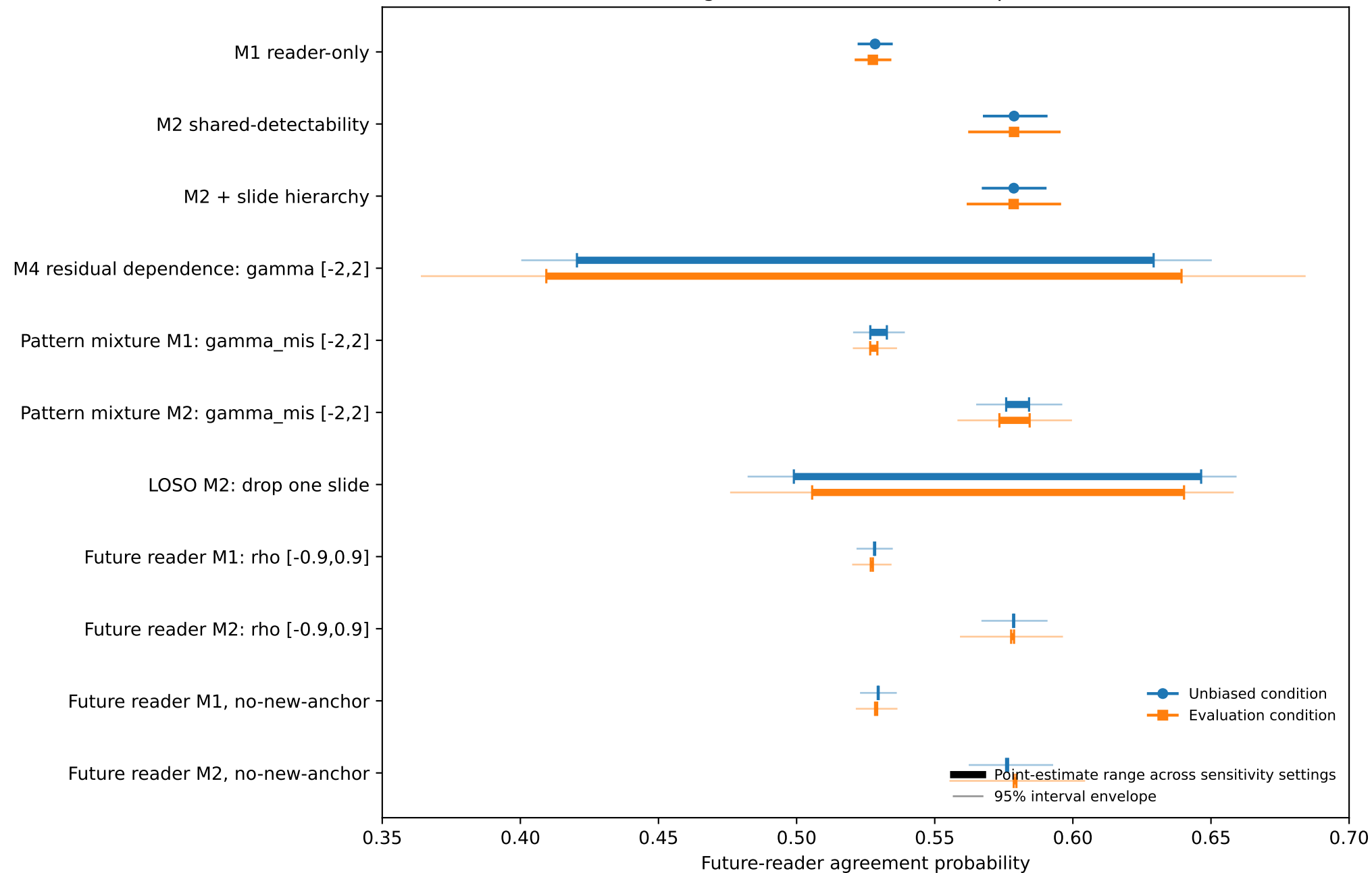
Absolute agreement under structural perturbations
