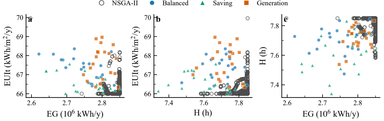
Figure 7: Pairwise objective-space comparison on the strict highest-accuracy 2000-sample surrogate. Each point is one candidate solution. The three DDPG scenarios still form overlapping clusters, while the fair-budget NSGA-II archive reaches stronger objective values on the same selected surrogate.
