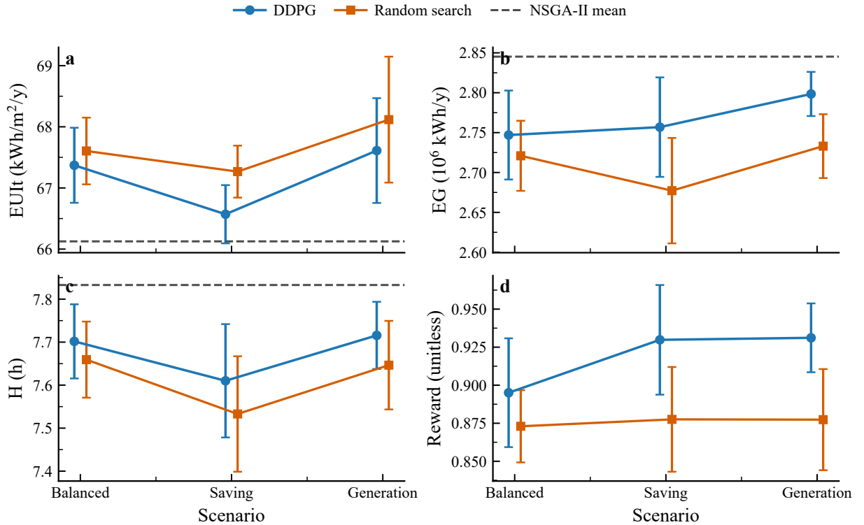
Figure 9: Accuracy-first benchmark summary on the strict highest-accuracy 2000-sample surrogate. Panels (a)–(c) compare scenario-wise objective summaries for DDPG and random search, with the NSGA-II mean shown as a dashed reference line. Panel (d) compares scalarized reward for DDPG and random search across the three scenarios.
