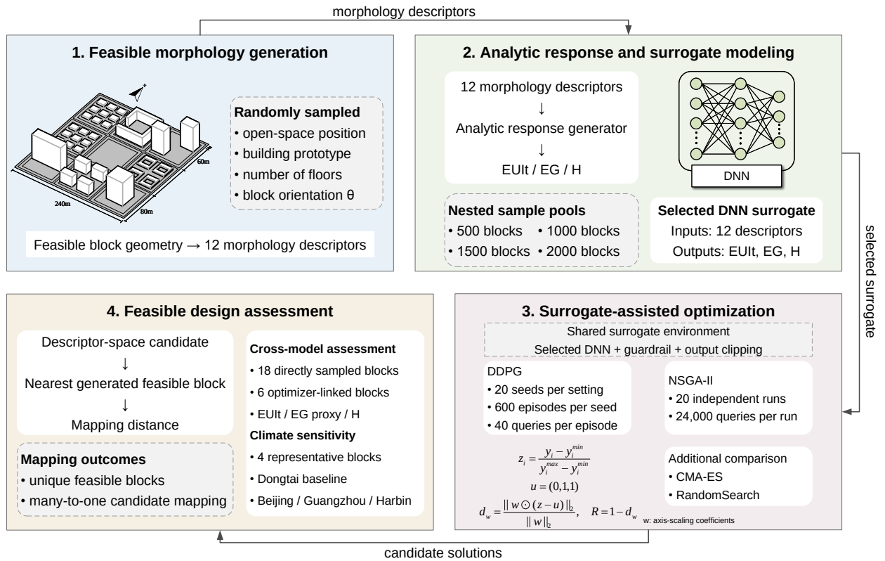
Figure 1: Workflow linking feasible morphology generation, analytic response assignment, surrogate-assisted optimization, feasible-block projection, and sensitivity analysis.
