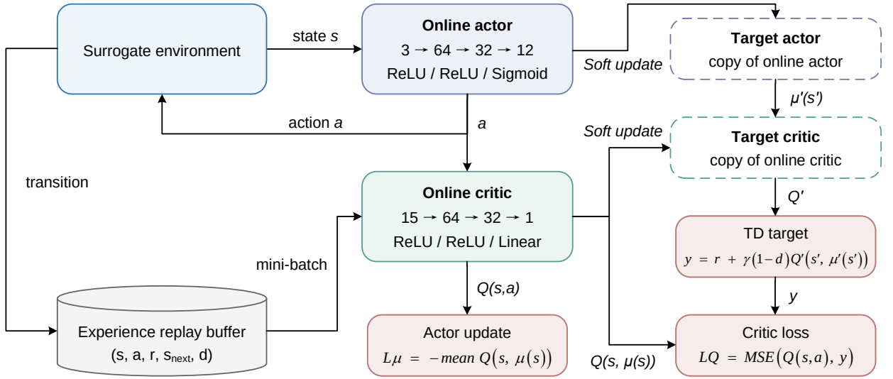
Figure 3: DDPG actor-critic architecture and target-network update structure used in the surrogate-query environment.
