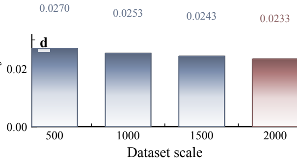
Selection objective
