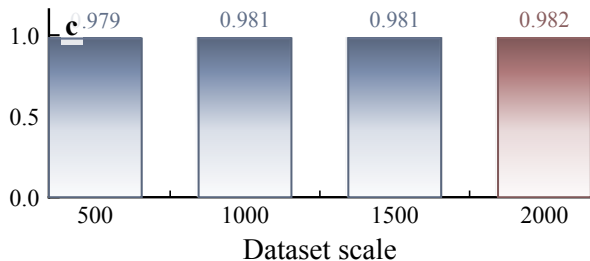
Mean R^2
